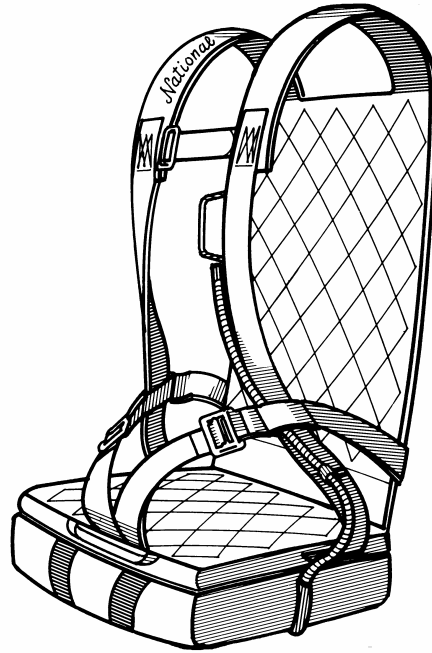
NATIONAL SEAT PARACHUTE (N-360-S / N-425-S / N-490-S)
