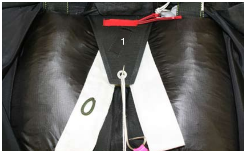
Figure 2-150. Pin The Closing Loop Above Flap 1
