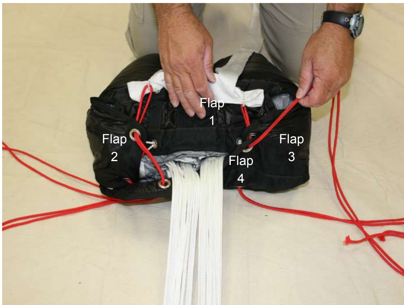
Figure 2-113. Close Flap 4
