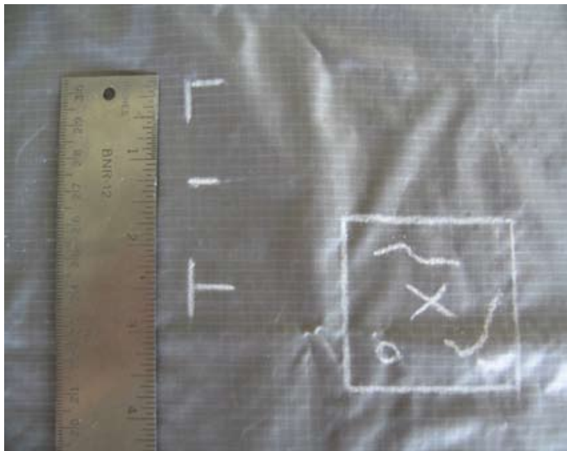
Figure 7-2. Determine Patch Layout
