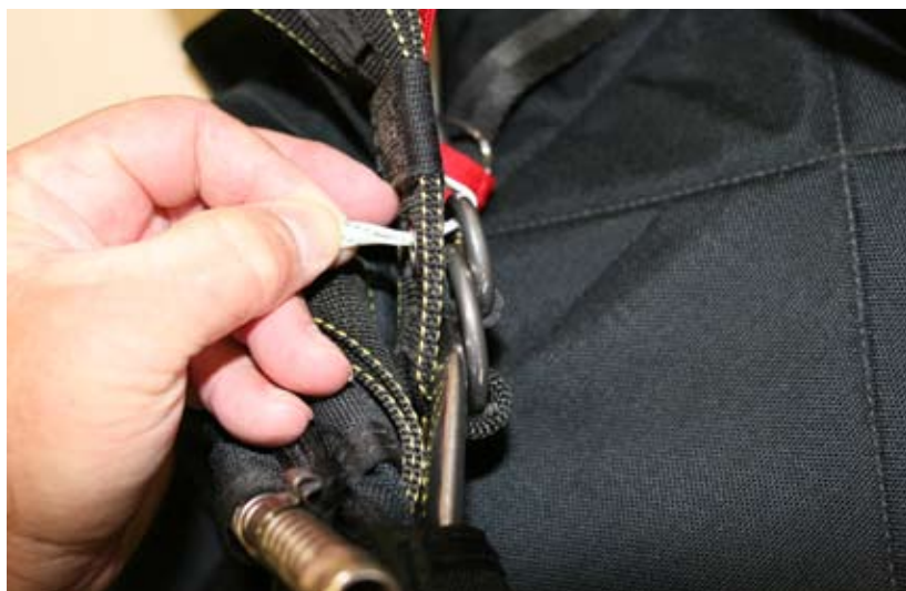
Figure 3-3. Insert Locking Loop Through The Riser
