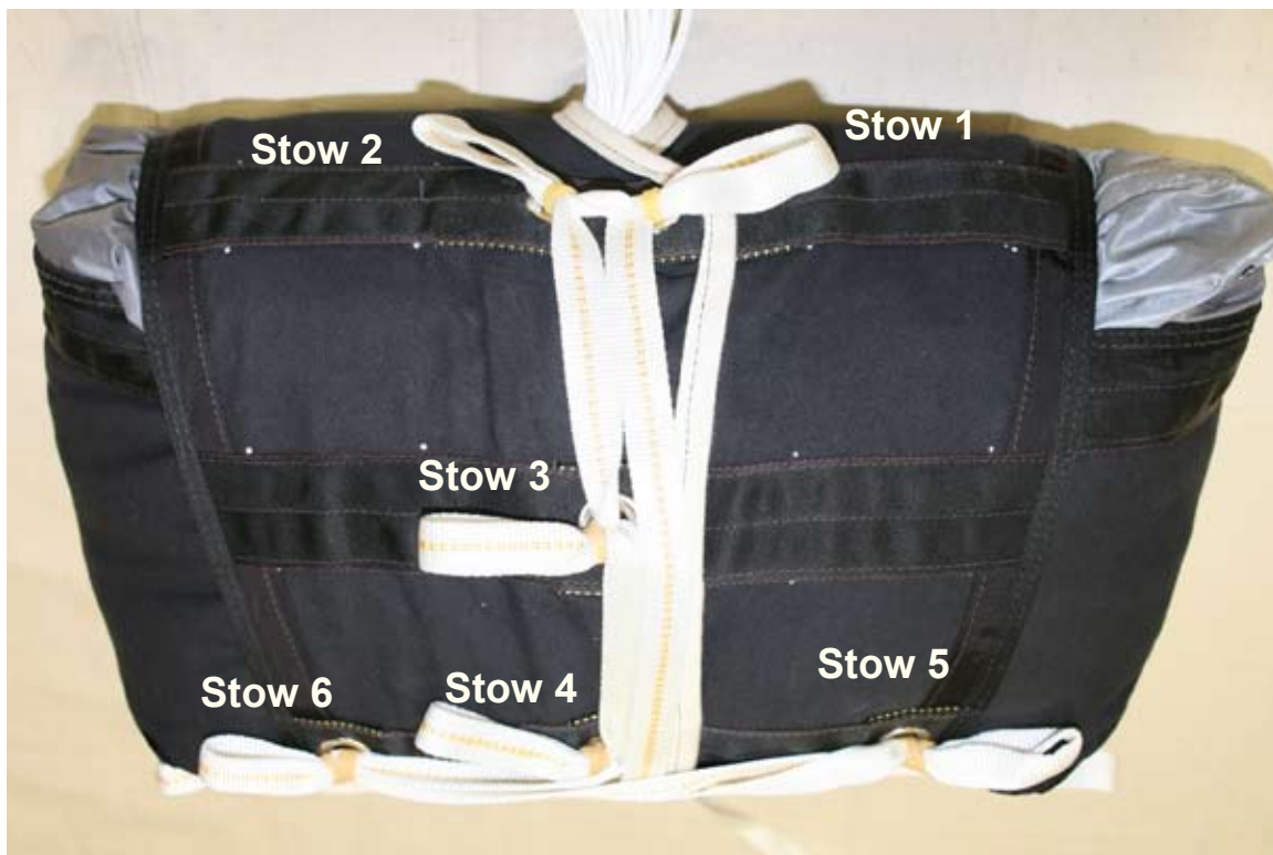
Figure 5-71. Complete The Locking Stow Sequence
