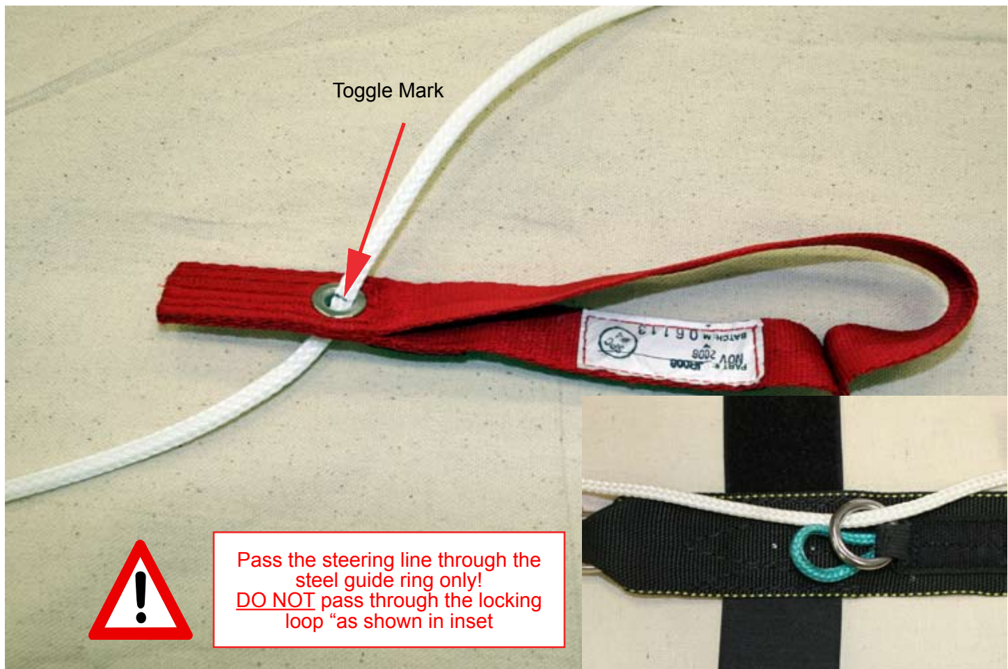
Figure 2-18. Thread Steering Line Through Steel Ring And Toggle Grommet
