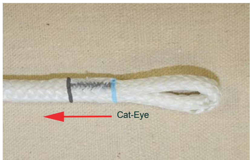
Figure 2-30. Finished Loop
