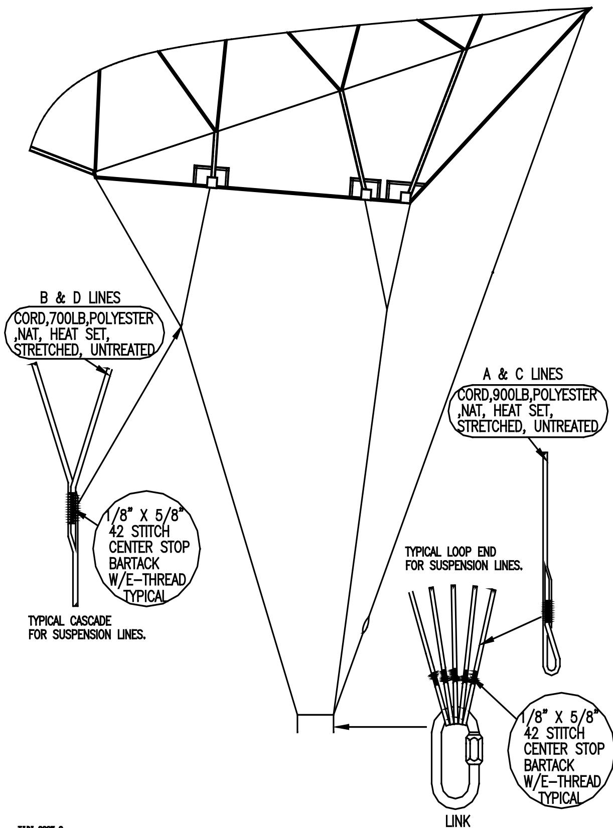
Figure 8-3. TR-375 Sideview
