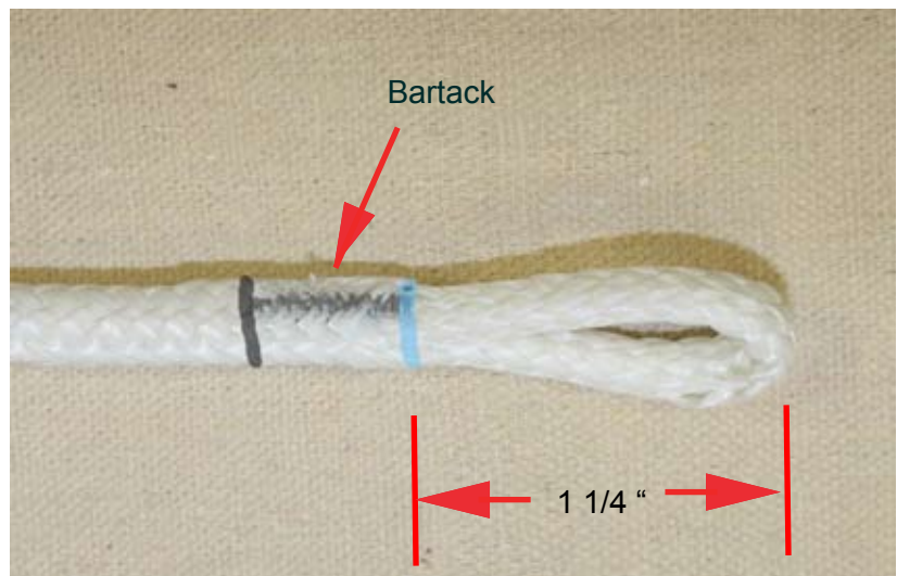
Figure 2-28. Completed Bartack
