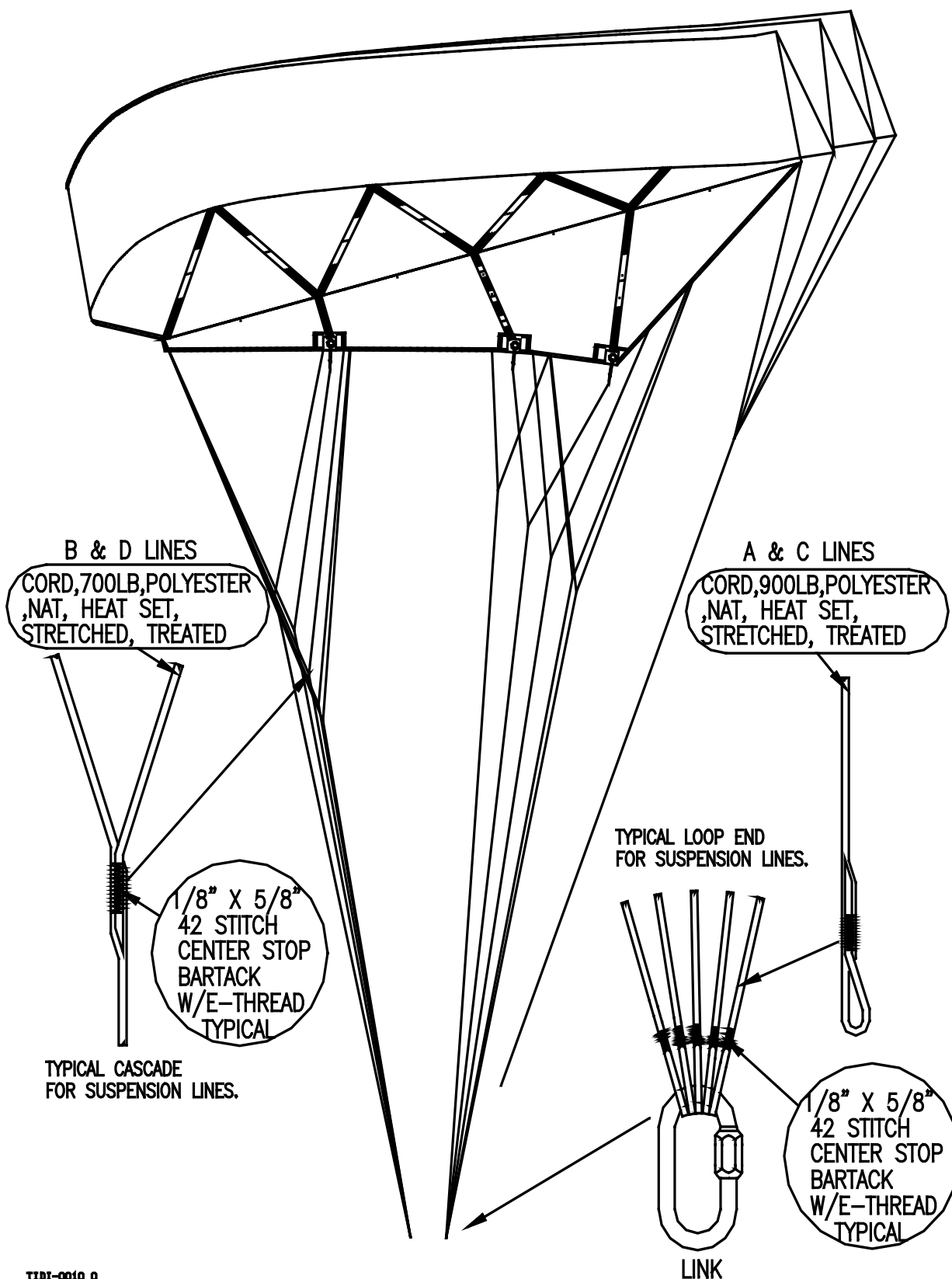
Figure 8-7. MS-360 Sideview
