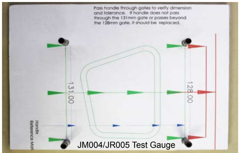
Figure 15. Test Gauge
